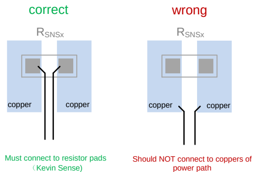
Current sense
