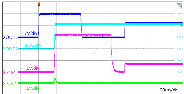
Figure 12-12 Short-to-battery Protection(Retry)
