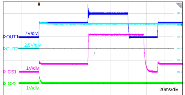
Figure 12-14 Reverse Current Protection(Retry)
