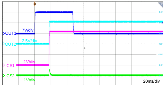
Figure 12-11 Short-to-battery Protection(Latch)
