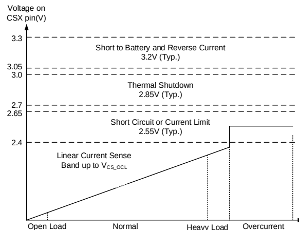
Figure 11-1 Current-sense Output and Its Multiplexing
