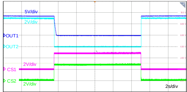
Figure 12-10 Thermal Shutdown Protection
