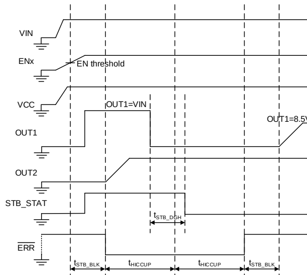
Figure 11-6 Auto-retry Mechanism_2
