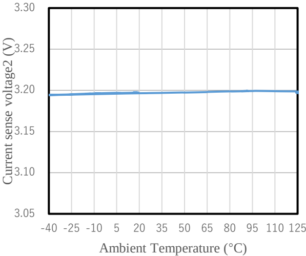
Figure 8-17 Current sense2 voltage at STB vs temperature
