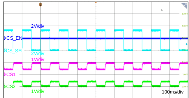
Figure 12-8 Current Sense Multiplexing
