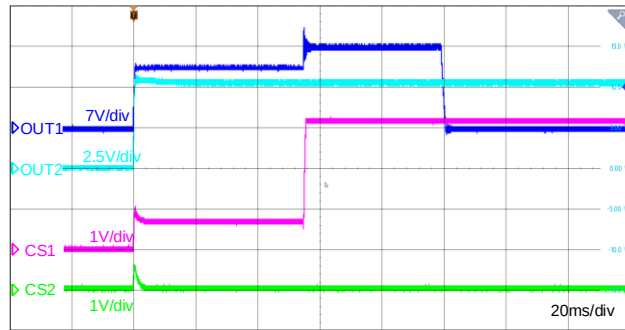
Figure 12-13 Reverse Current Protection(Latch)
