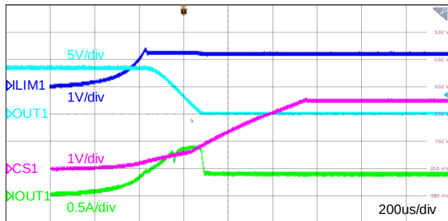
Figure 12-9 Current Limit
