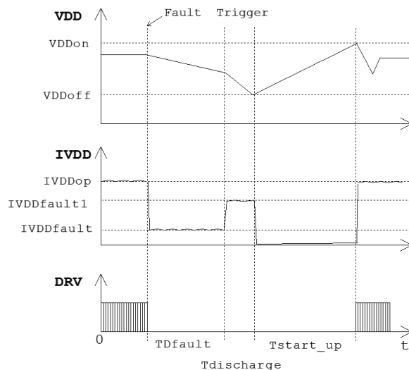
Fig. 9 Auto-Recovery Process
