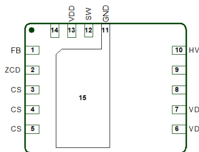
Fig. 2 Top view
