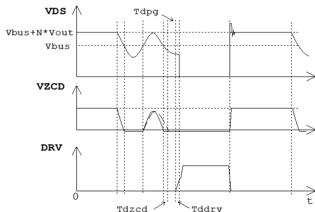
Fig. 8 Valley Switching
