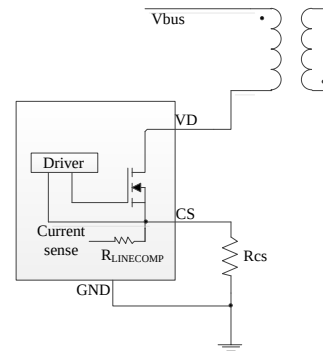
Fig. 7 current sense
