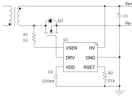
Figure.2 SC3520 Typical Application circuit (low side)
