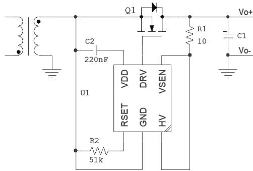
Figure.1 SC3520 Typical Application circuit (high side)
