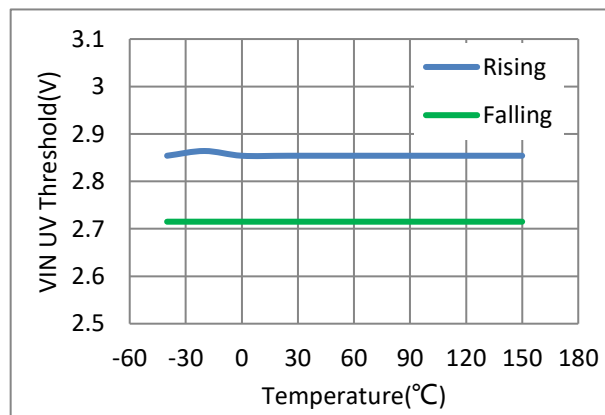
Figure 8-6 VIN UV Threshold
