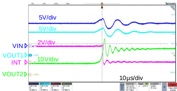
Figure 8-11. OUT1=50 \Omega , OUT2 Short to 28V Battery
