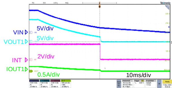
Figure 8-8. V_{IN} OFF, OUT1=50 \Omega
