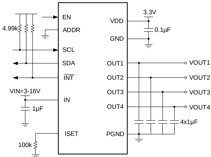
Figure 6-1. Typical Application Circuit of SC71440XQ
