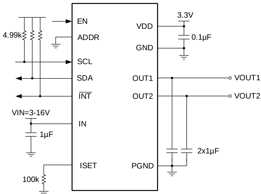
Figure 6-2. Typical Application Circuit of SC71240AQ
