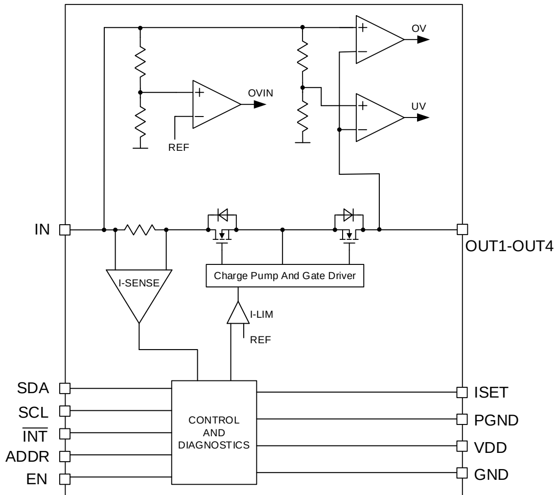
Figure 9-1. Function Block
