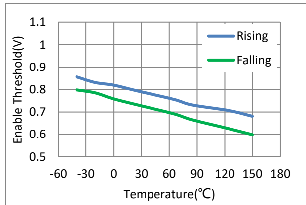
Figure 8-5 Enable Threshold
