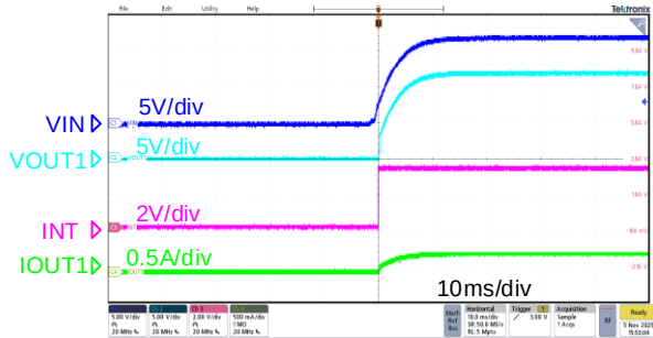
Figure 8-7. V_{IN} ON, OUT1=50 \Omega
