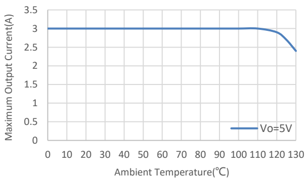
Figure 11-15. Maximum Output Current versus Ambient Temperature(Base on demo)
