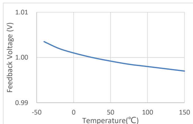
Figure 8-6. Feedback Voltage
