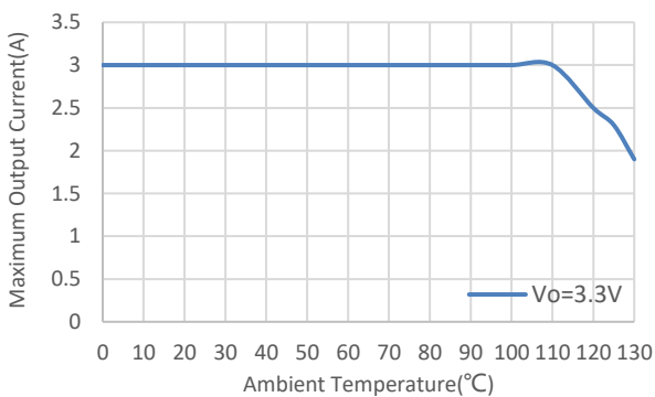
Figure 11-16. Maximum Output Current versus Ambient Temperature
