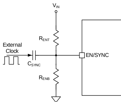
Figure 10-4 EN/SYNC Configuration for Clock Synchronization
