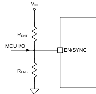
Figure 10-3 EN/SYNC Configuration for Precise Enable
