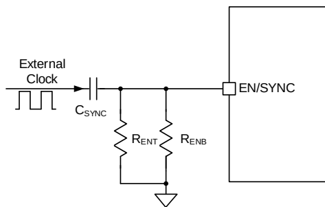
Figure 10-5 EN/SYNC High-pass Filter Demonstration
