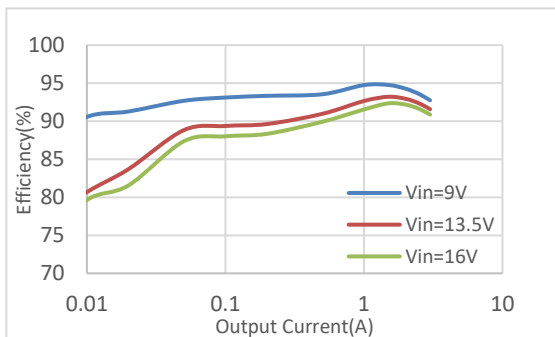
Figure 11-1. Efficiency Curves
