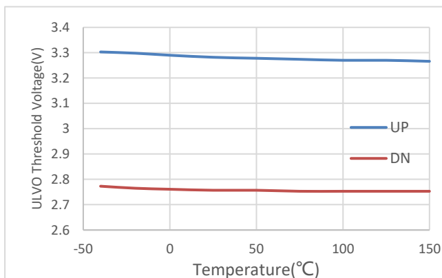
Figure 8-5. UVLO Thresholds
