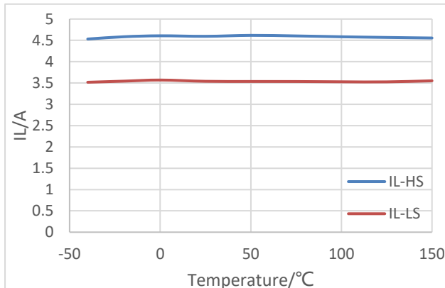
Figure 8-3. \text{IL-HS} and \text{IL-LS} Output Current
