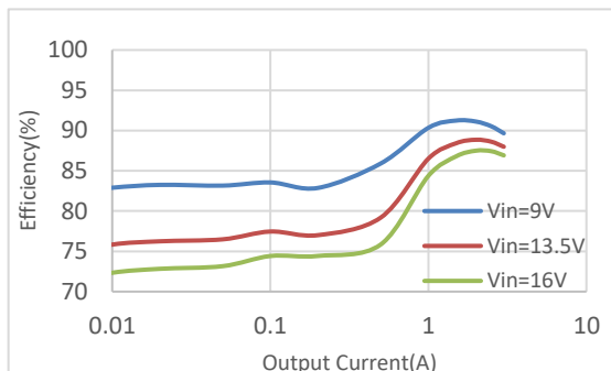
Figure 11-2. Efficiency Curves
