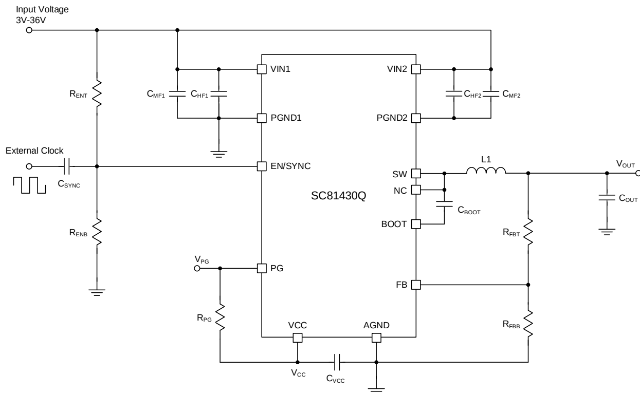
Figure 6-1. Typical Application Circuit of SC81430Q
