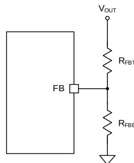
Figure 10-1 FB Configuration
