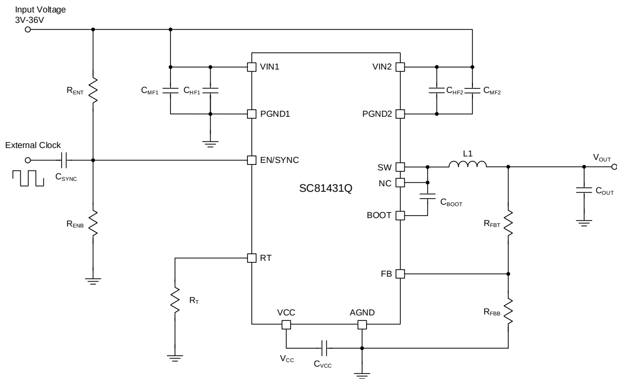
Figure 6-2. Typical Application Circuit of SC81431Q/ SC81431AQ
