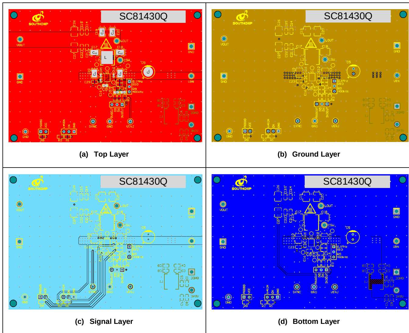
Figure 12-1. Layout Example
