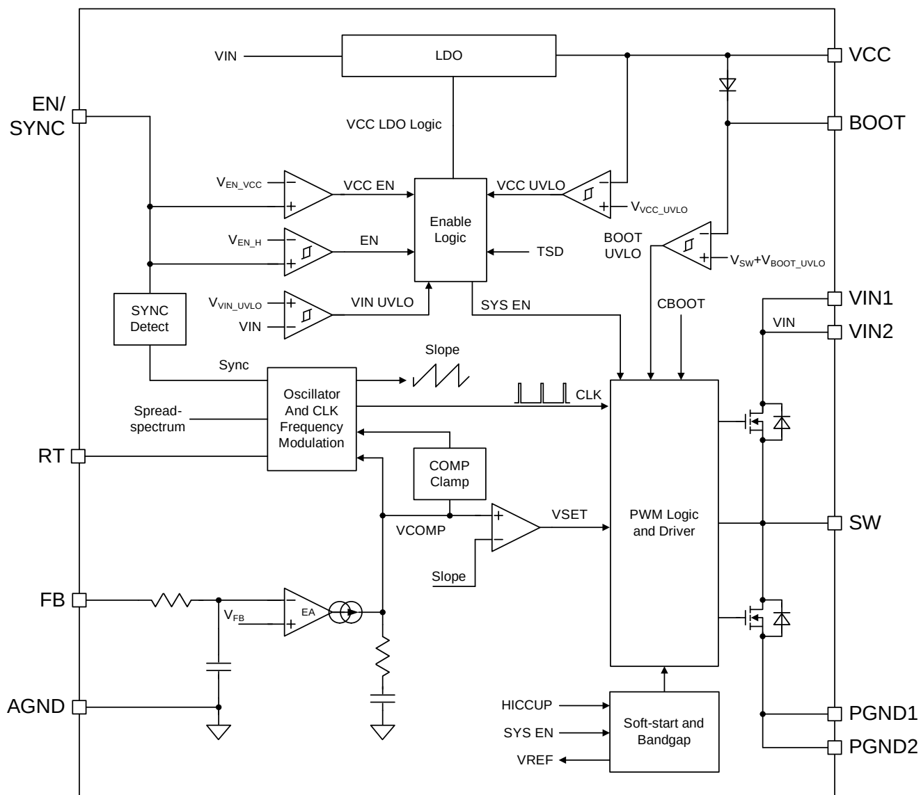
Figure 9-2. SC81431Q, SC81431AQ Functional Block Diagram
