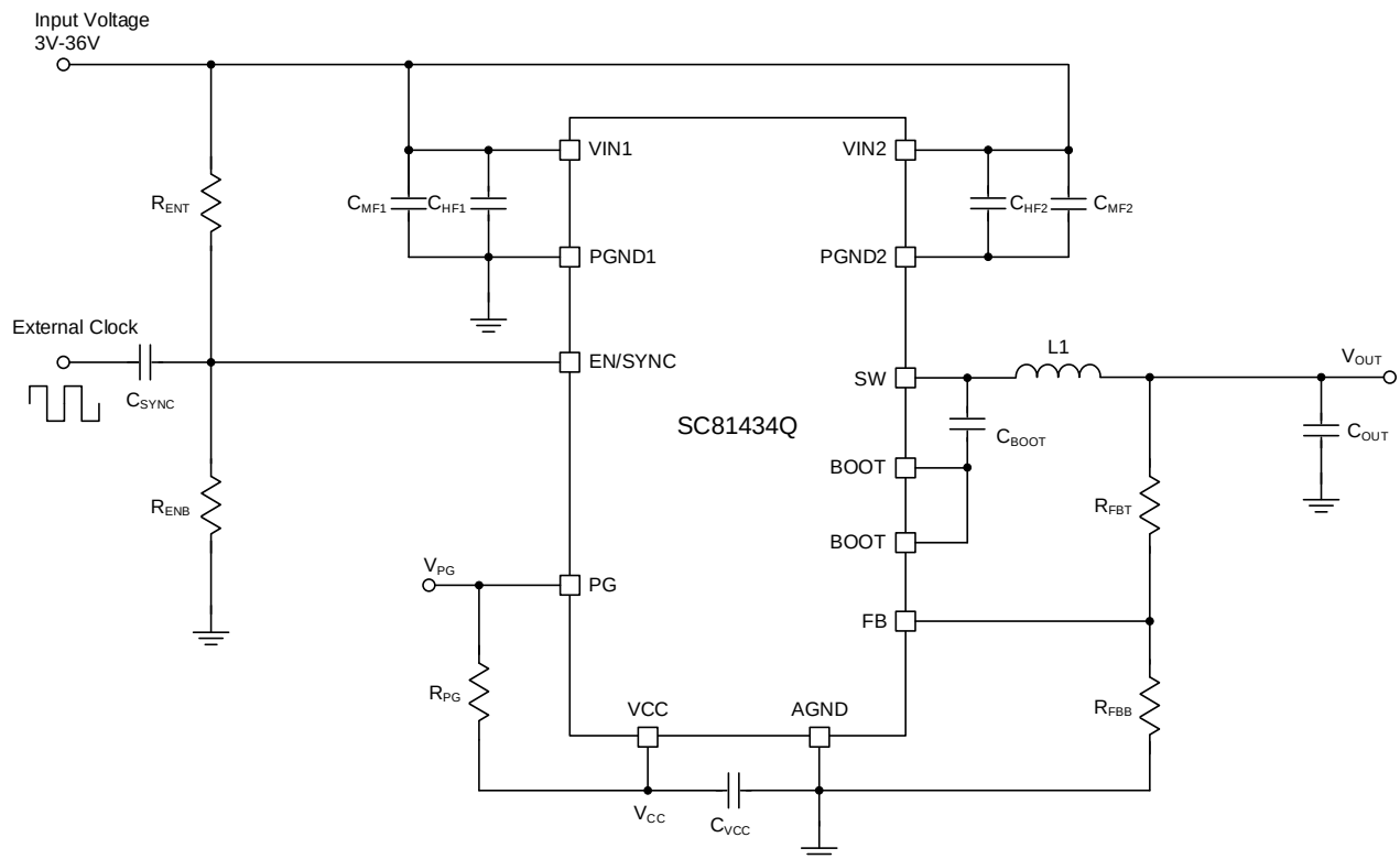
Figure 6-3. Typical Application Circuit of SC81434Q/ SC81434BQ
