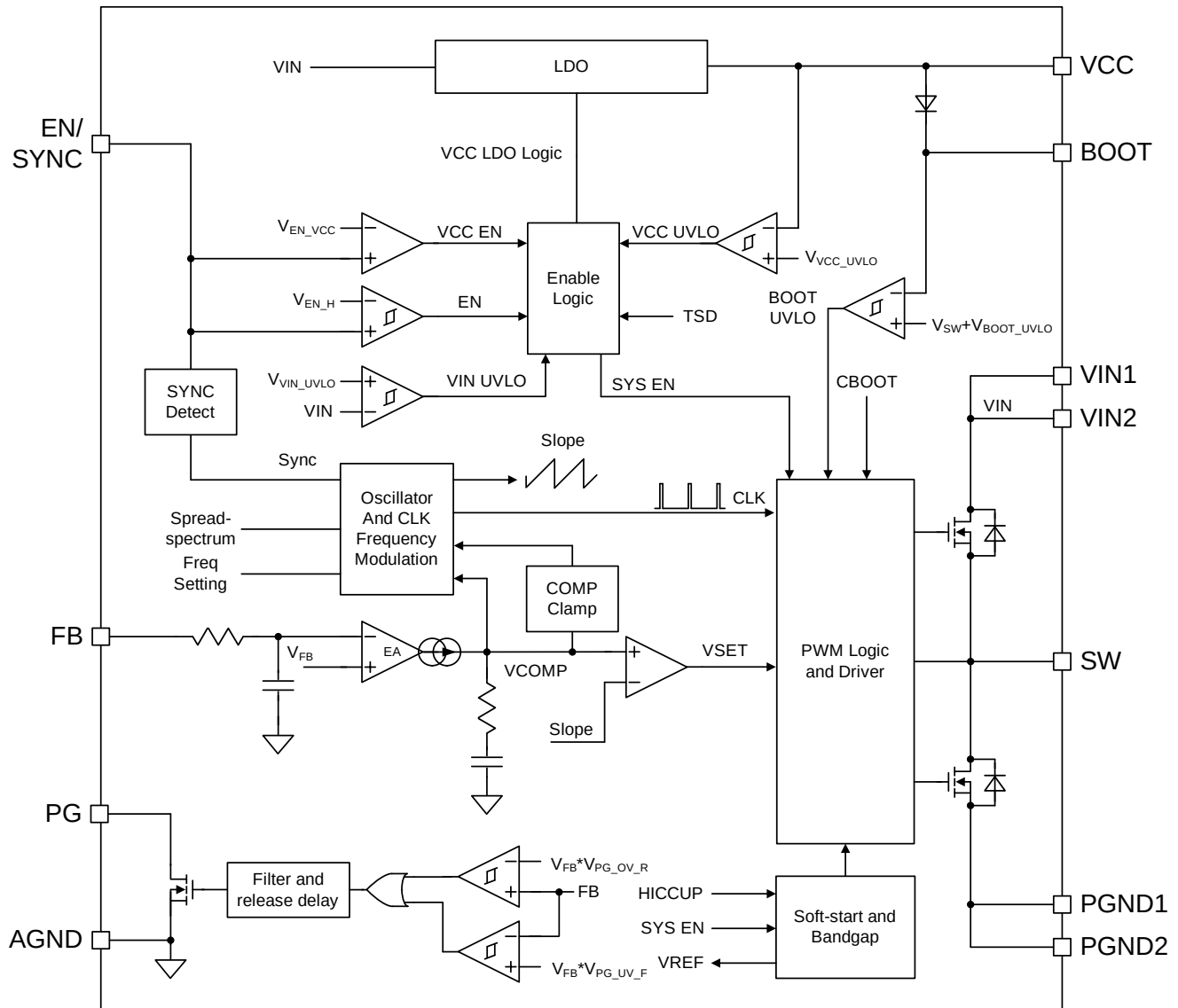
Figure 9-1. SC81430Q, SC81434Q and SC81434BQ Functional Block Diagram
