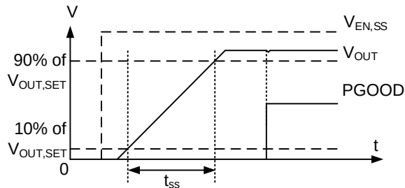
Figure 10-8 Soft-start With No Pre-bias
