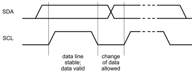
Figure 2 Bit transfer on the I2C bus
