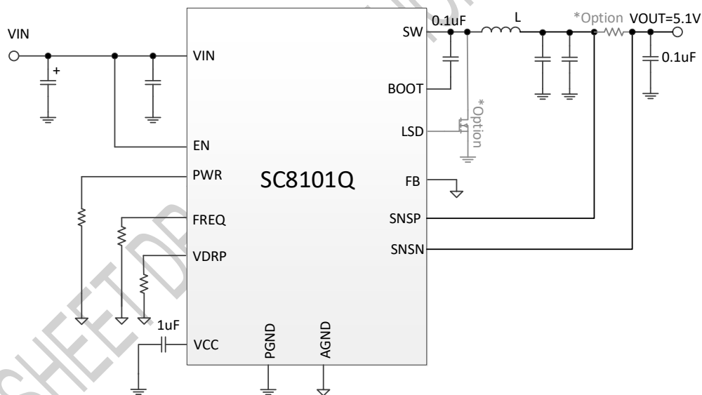
Figure.2 Typical application with 5.1V output
