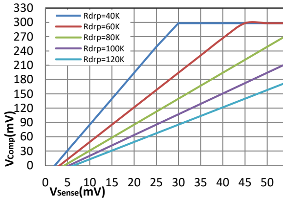
Figure.5 5 V_{COMP} vs. V_{SENSE} ( R_U=78.5 K \Omega )
