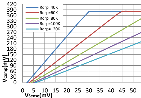
Figure.6 5 V_{COMP} vs. V_{SENSE} ( R_U=100 K \Omega )
