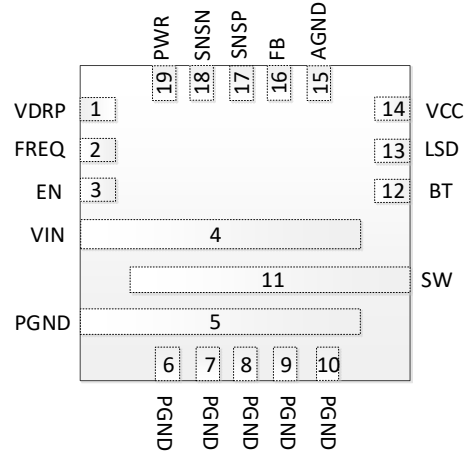
QFN 19 Package Reference (Top View)
