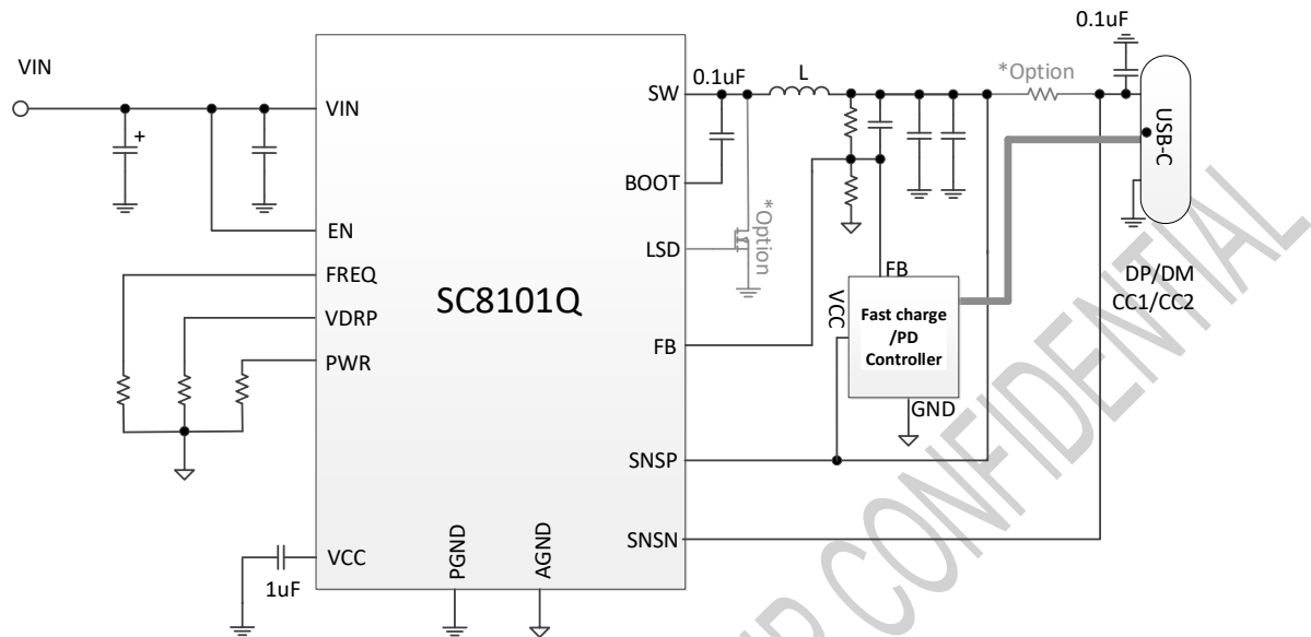
Figure.1 Typical Application Circuit for Fast charge/PD Application
