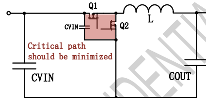
Figure.7 Minimizing the critical path helps mitigate EMI
