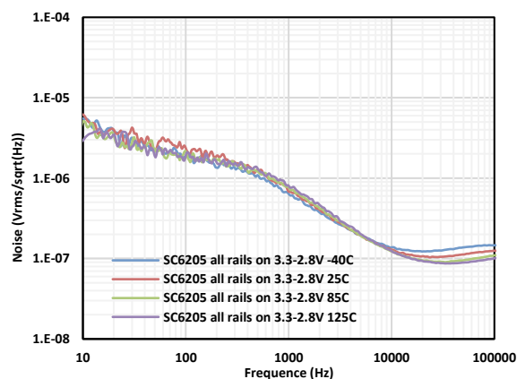
Figure11-8, LDO Output Noise, IO4=300mA
