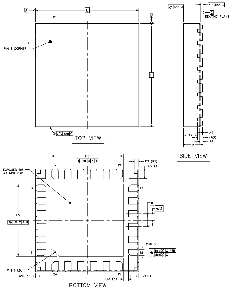
QFN-24-4mm*4mm Wettable Flank
