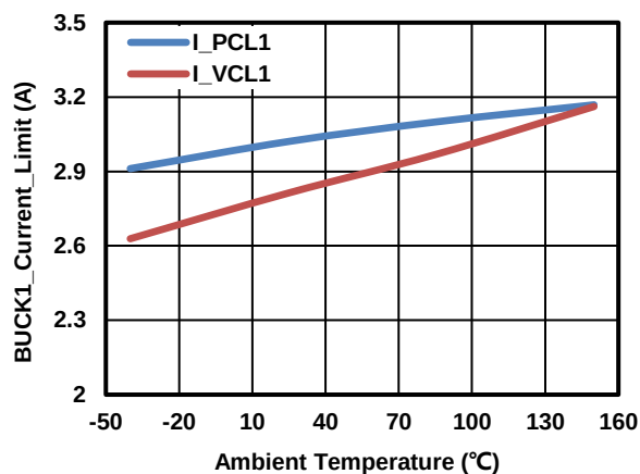
Figure 8-6, BUCK1_Current_Limit vs Temperature
