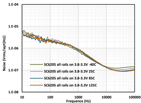
Figure11-7, LDO Output Noise, IO4=300mA
