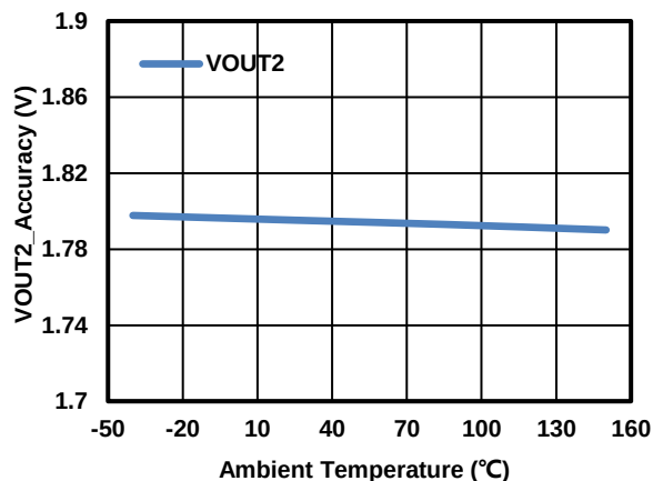
Figure 8-10, VOUT2_Accuracy vs Temperature
