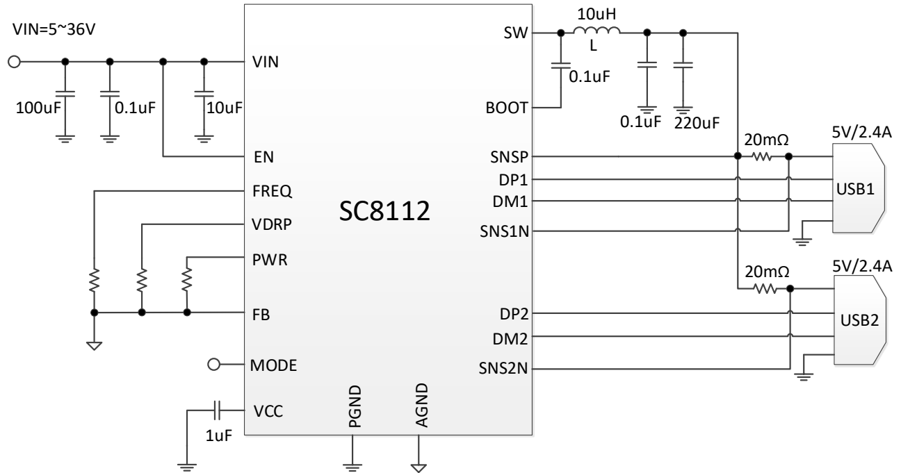
Figure. 1 Typical Application Circuit with 5V4.8A Dual-Outputs
