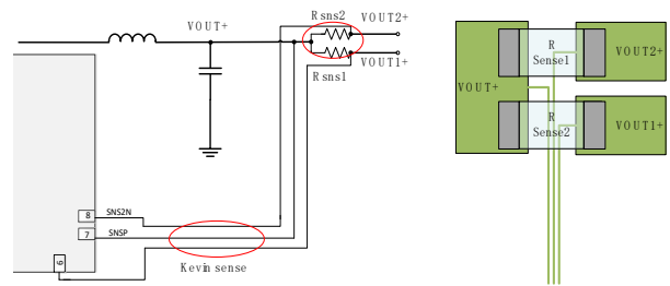
Figure.10 Current sense
