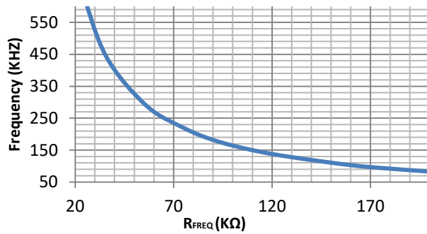
Figure.4 Switching Frequency vs. Setting Resistor
