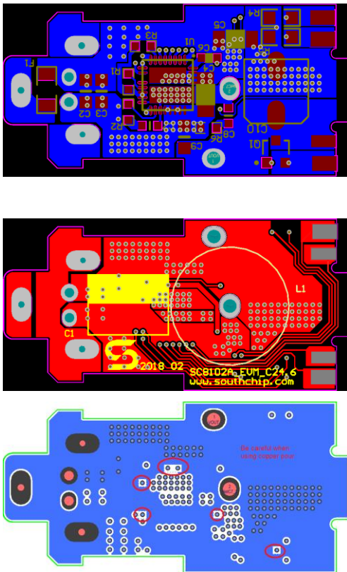
Figure.8 Reference design
