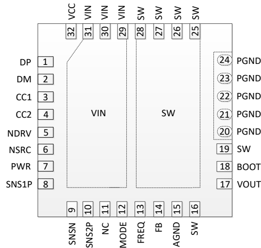
QFN 32 Package Reference
