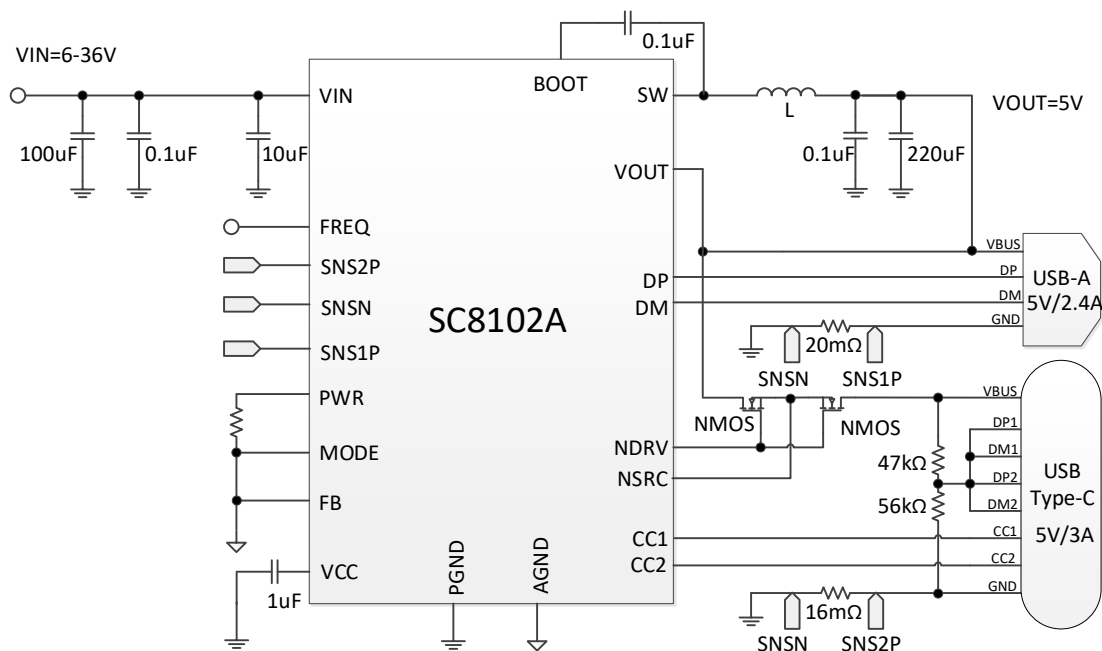
Figure.2 Typical Application Circuit with Dual-Outputs and Back-to-Back Isolated NMOS
