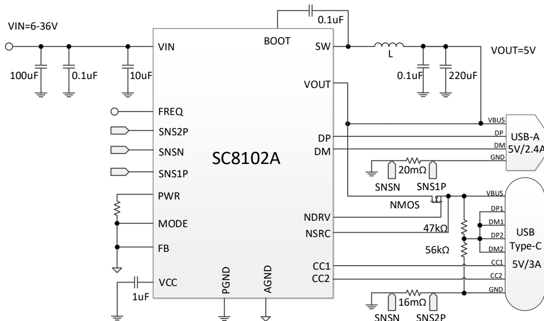
Figure.1 Typical Application Circuit with Dual-Outputs and Isolated NMOS
