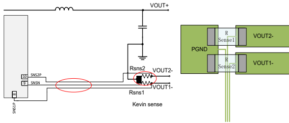
Figure.7 Current sense
