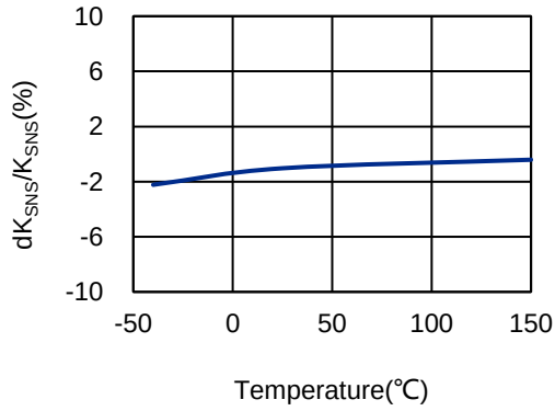
Figure 8-11. dK_{sns} / K_{sns} vs T_A ( I_{OUT} = 0.05A )
