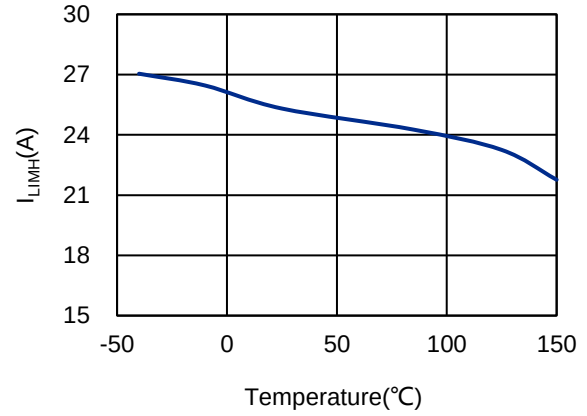
Figure 8-10. I_{LIMH} vs T_A
