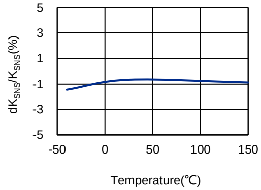
Figure 8-12. dK_{sns} / K_{sns} vs T_A ( I_{OUT} = 3A )
