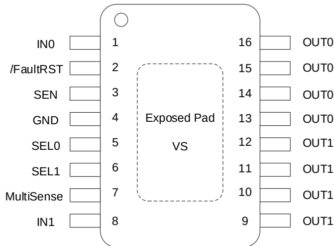
Figure 7-1. Configuration Diagram (Top View)
