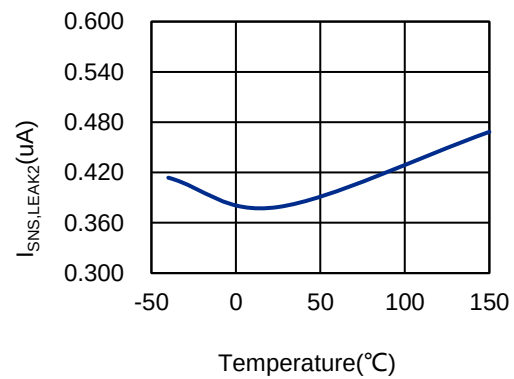
Figure 8-14. I_{SNS,LEAK2} vs T_A
