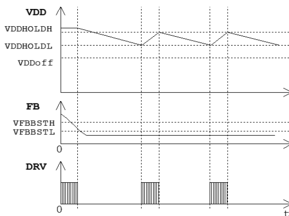
Fig. 4 VDD holding circuitry
