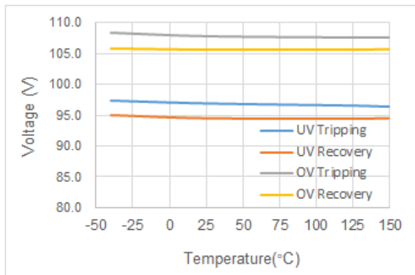
Figure 8-8. PGOOD Thresholds
