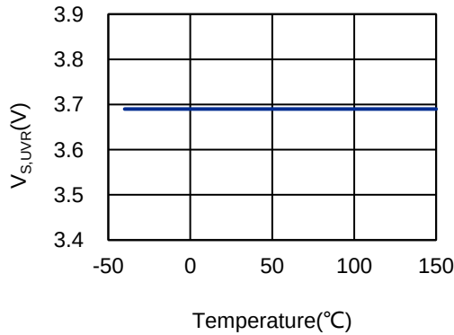
Figure 8-1. V_{S,UVR} vs T_A
