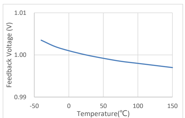
Figure 8-6. Feedback Voltage
