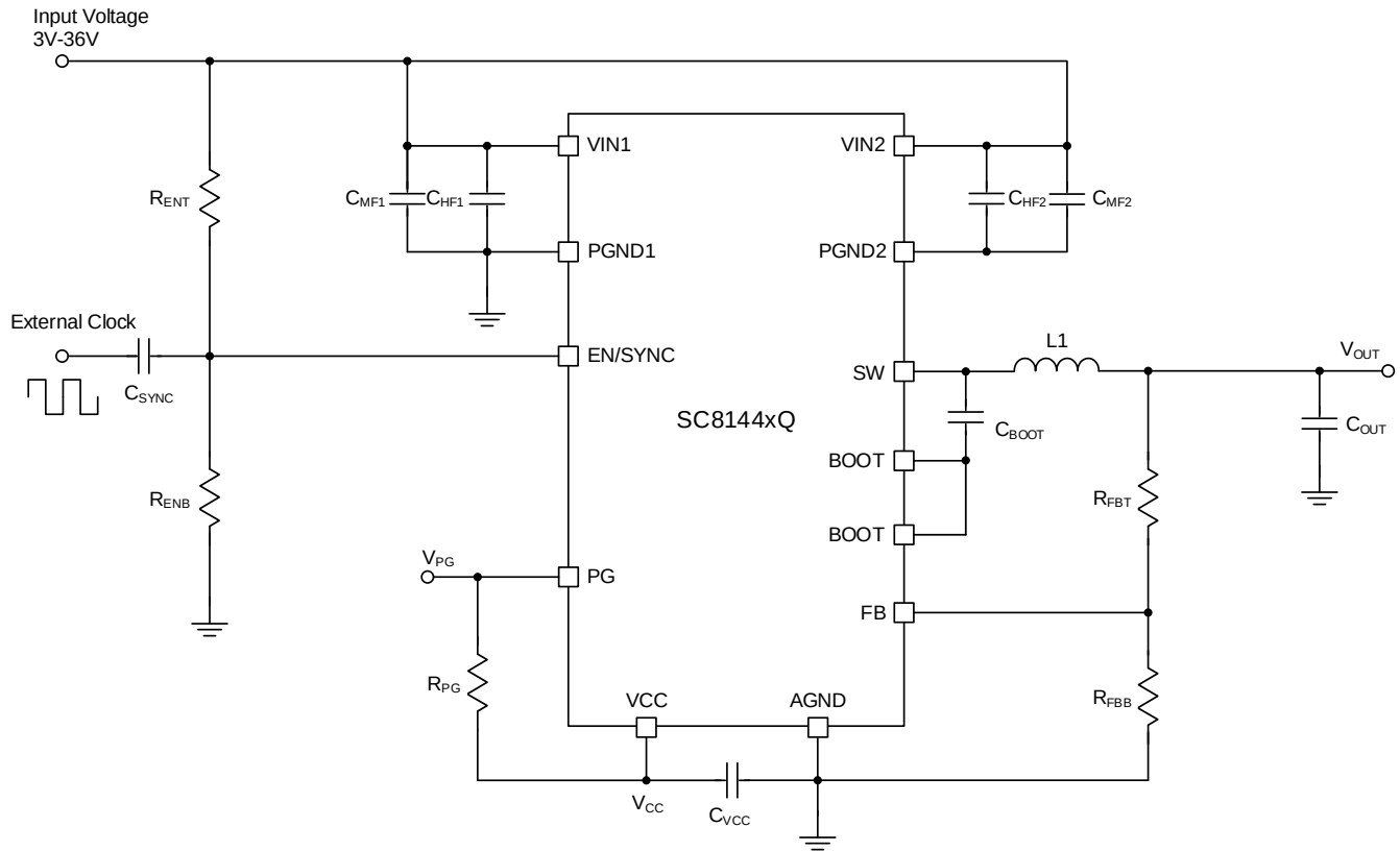
Figure 6-1. Typical Application Circuit of SC81444Q/SC81444AQ
