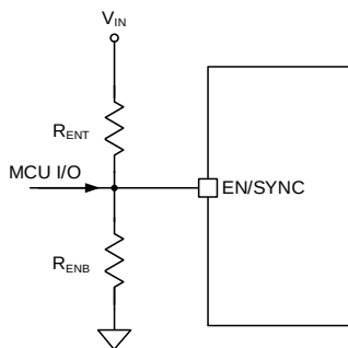
Figure 10-2 EN/SYNC Configuration for Precise Enable
