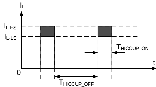
Figure 10-6 Hiccup Mode Operation
