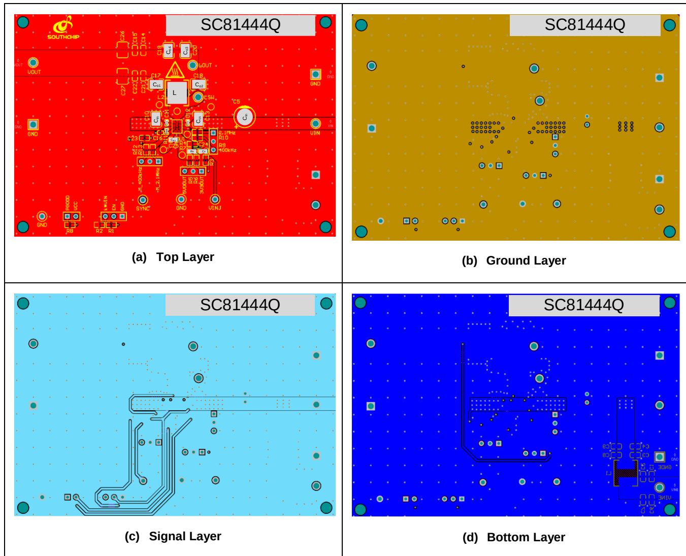
Figure 12-1. Layout Example
