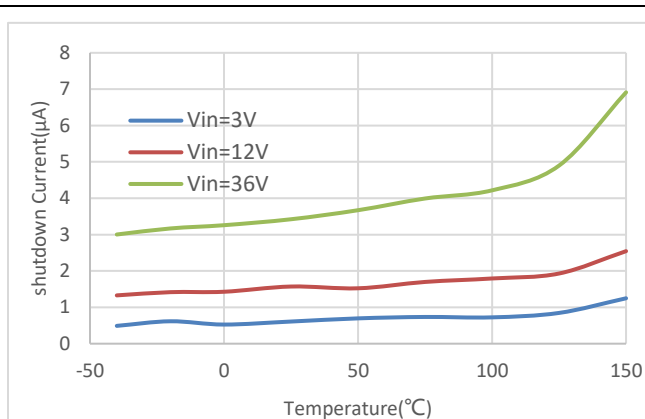
Figure 8-2. Shutdown Supply Current
