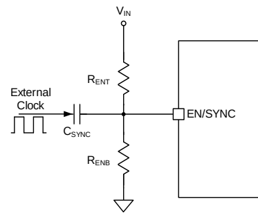
Figure 10-3 EN/SYNC Configuration for Clock Synchronization
