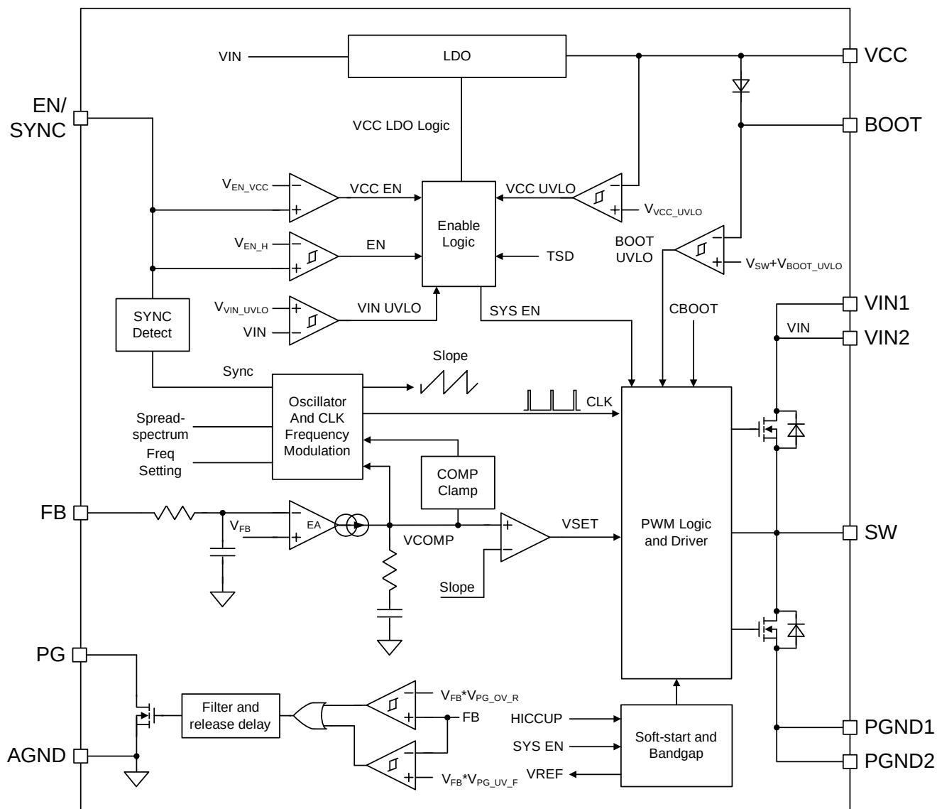
Figure 9-1. SC81444Q and SC81444AQ Functional Block Diagram
