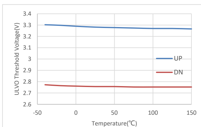
Figure 8-5. UVLO Thresholds
