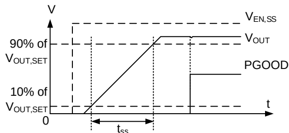
Figure 10-7 Soft-start With No Pre-bias
