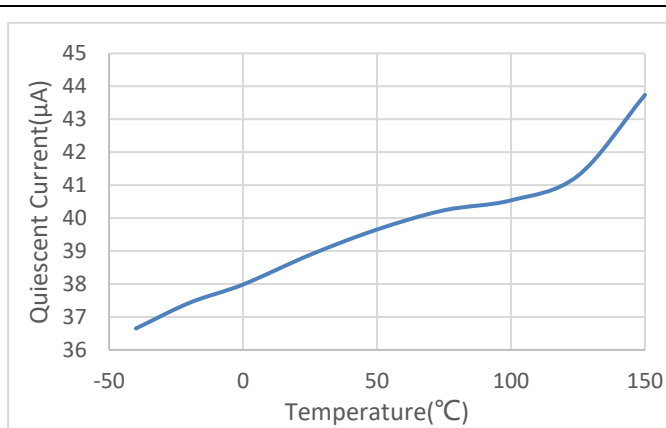
Figure 8-1. Non-Switching Input Supply Current
