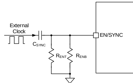
Figure 10-4 EN/SYNC High-pass Filter Demonstration
