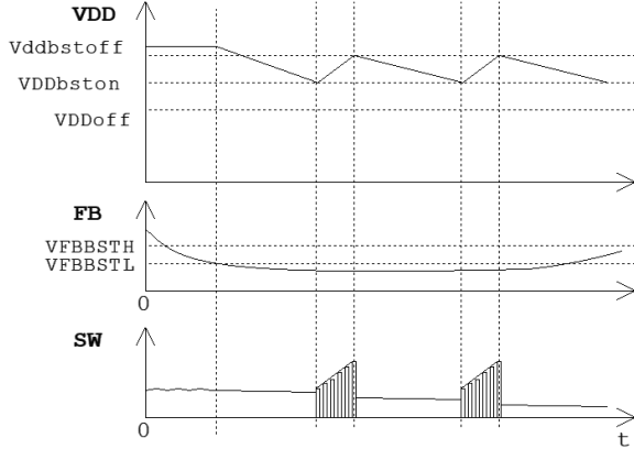
Fig. 5 The Boost Circuit
