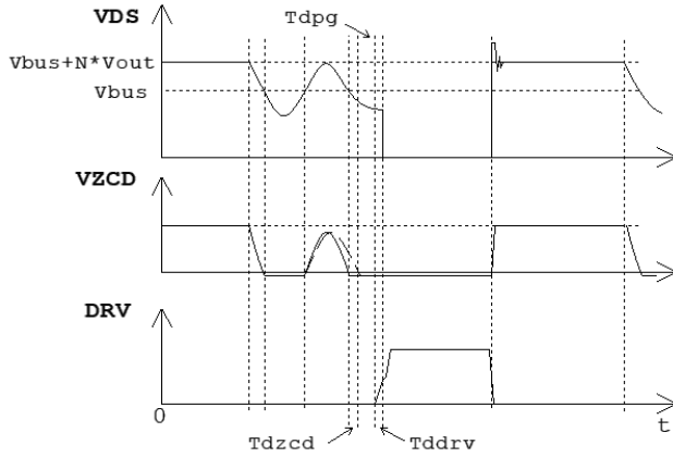
Fig. 7 Valley Switching
