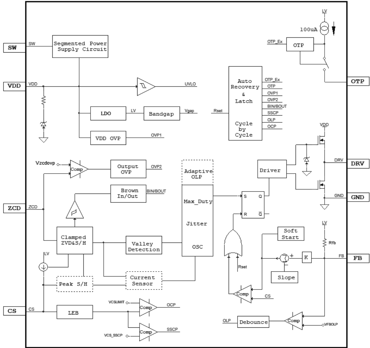
Fig.3 Function Block Diagram
