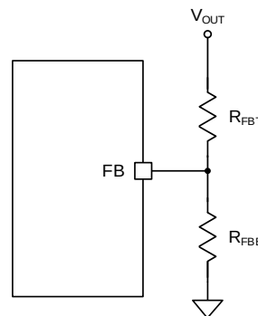
Figure 10-1 FB Configuration
