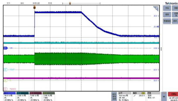
Suppressed Load Dump Test
