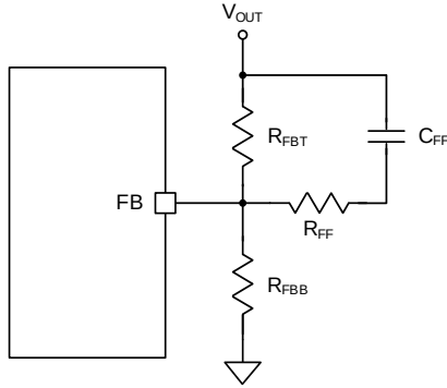
Figure 10-2 FB Configuration with Feedforward Network
