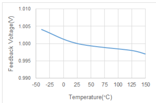
Figure 8-3. Feedback Voltage
