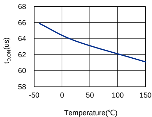
Figure 8-8. t_{D,ON} vs T_A
