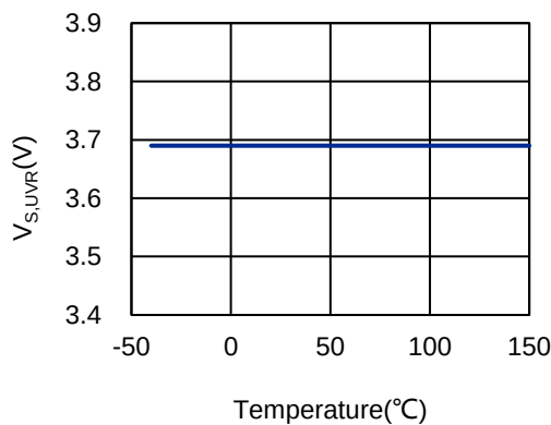
Figure 8-1. V_{S,UVR} vs T_A
