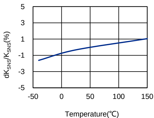
Figure 8-12. dK_{SNS} / K_{SNS} vs T_A ( I_{OUT} = 5\text{A} )
