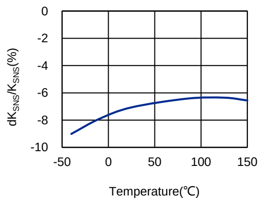
Figure 8-11. dK_{SNS} / K_{SNS} vs T_A ( I_{OUT} = 0.01\text{A} )
