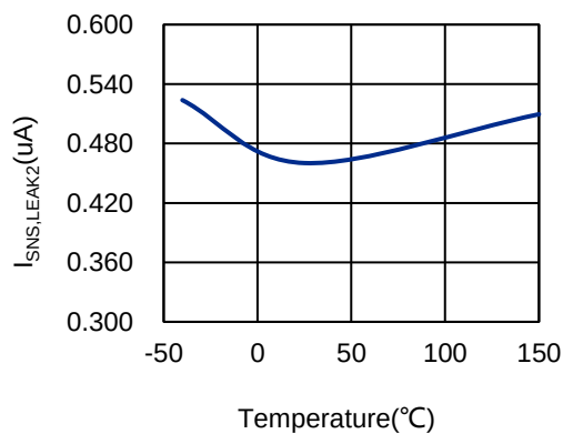
Figure 8-14. I_{SNS,LEAK2} vs T_A
