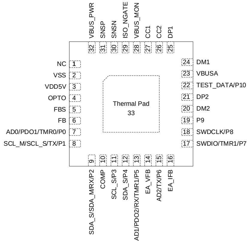
TOP VIEW of SC2021Q (QFN-32)
