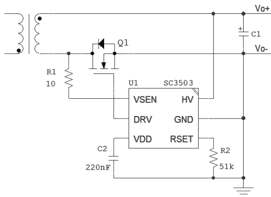
For High V_{GS} MOSFET ( V_{DD\_REG}=8.0V )
