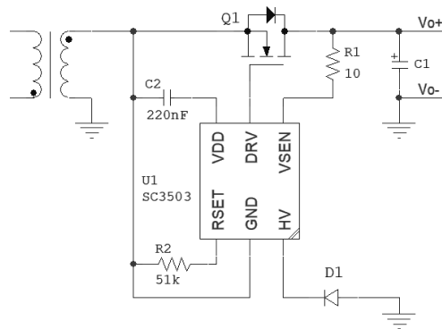
For High output voltage ( V_{DD\_REG}=8.0V )
