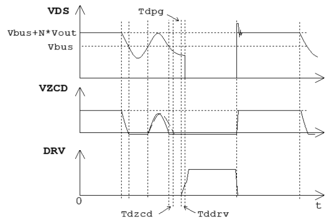
Fig. 7 Valley Switching
