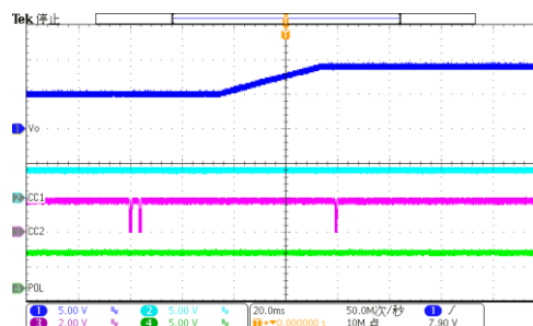
Figure 8-44. PDO Transition 5V-9V
