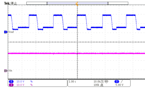
Figure 8-52. VOUT Short to 18V Battery
