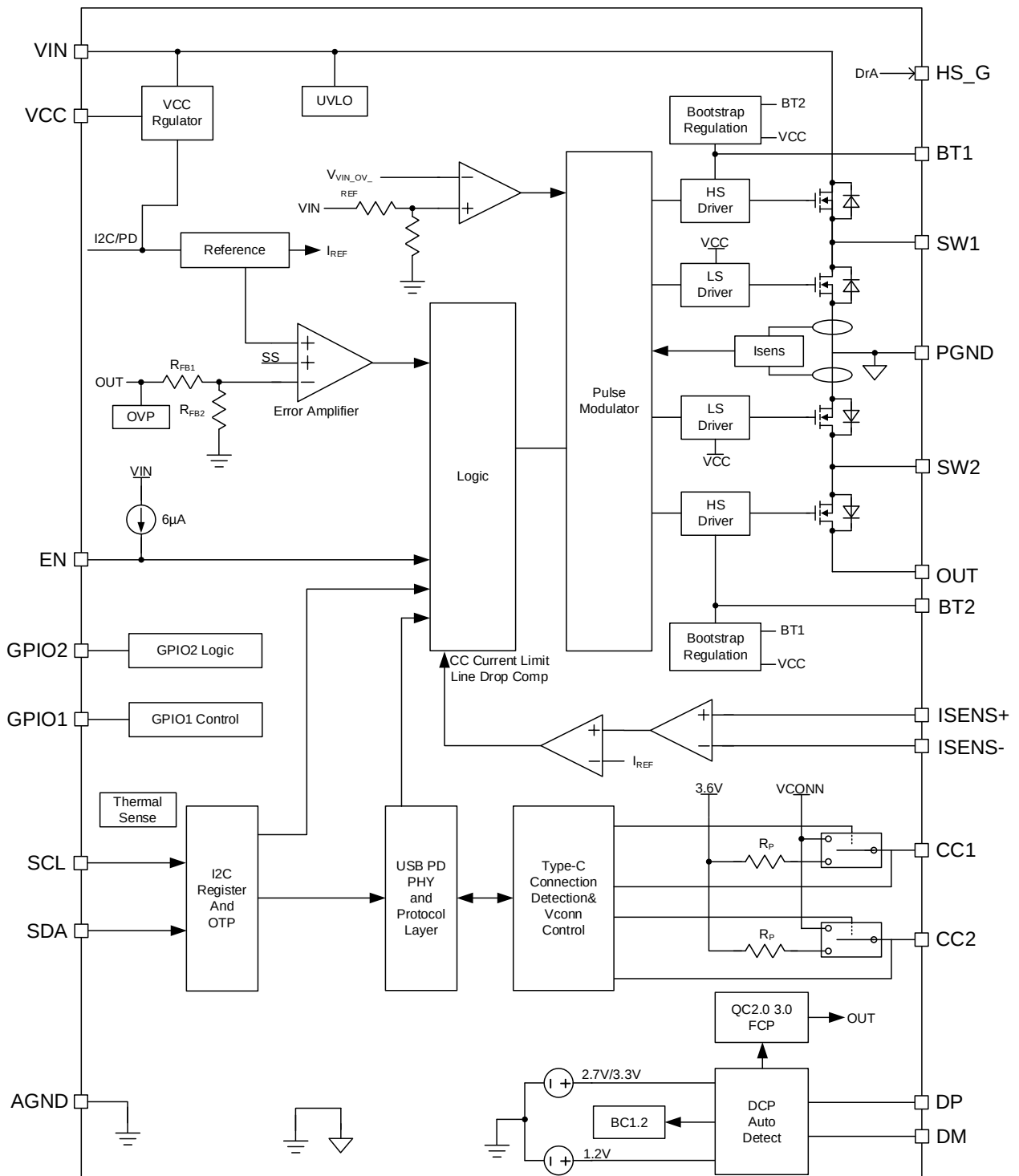
Figure 9-1. Function Block
