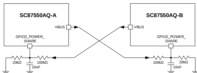
Figure 10-5 GPIO2 Power Share Connection Between Two SC87550AQs
