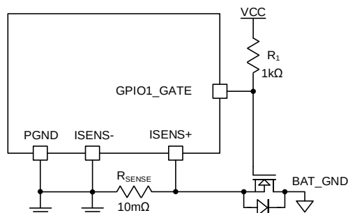
Figure 10-3 Battery Short-to-Ground Driver
