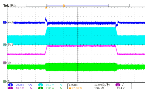
Figure 8-42. Line Transient, V_{IN}=9-18V , V_{OUT}=5V , I_{OUT}=3A
