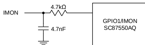
Figure 10-2 IMON Connection
