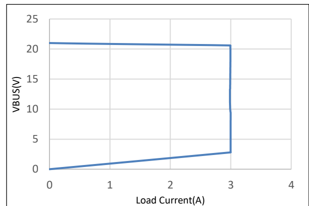
Figure 8-6. CC/CV Curve
