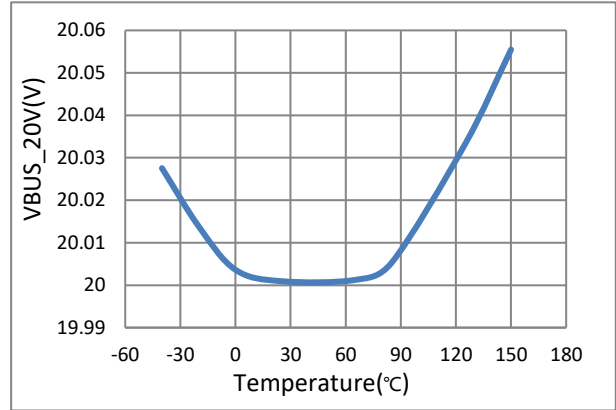
Figure 8-8. V BUS Voltage-20V
