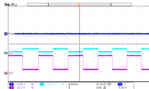
Figure 8-56. CC2 Short to 18V Battery (Detach)
