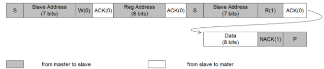
Figure 10-12. Single Read
