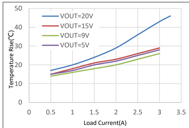
Figure 8-1. Case Temperature Rise, disable external Q1, DCR=9mR
