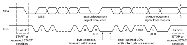
Figure 10-8. Data transfer on the I2C bus
