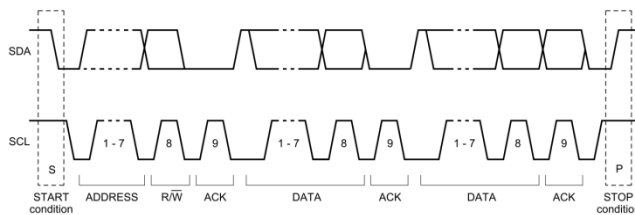
Figure 10-9. complete data transfer
