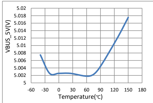
Figure 8-9. V BUS Voltage-5V
