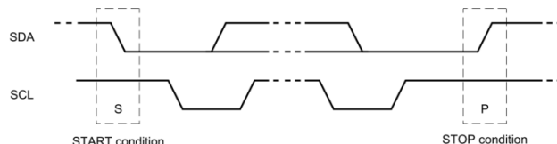
Figure 10-7. START and STOP conditions
