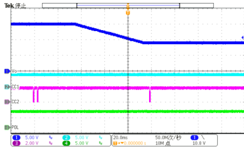
Figure 8-47. PDO Transition 15V-9V
