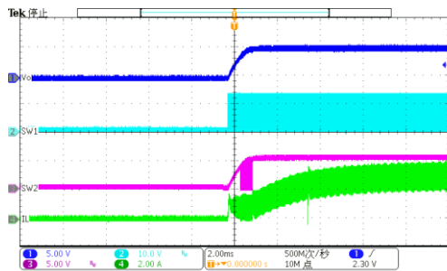
Figure 8-35. Start up through V_{IN} ; I_{OUT} = 3A
