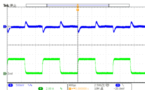
Figure 8-40. Load Transient, V_{OUT}=5V , I_{OUT}=0-3A
