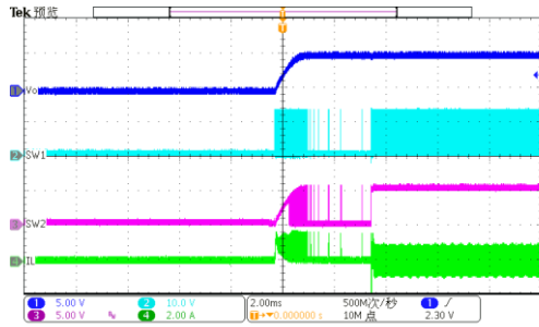
Figure 8-33. Start up through V_{IN} ; I_{OUT} = 0A
