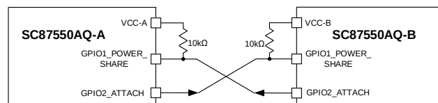
Figure 10-4 GPIO1 Power Share Connection Between Two SC87550AQs
