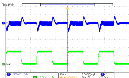
Figure 8-41. Load Transient, V_{OUT}=20V , I_{OUT}=0-3A
