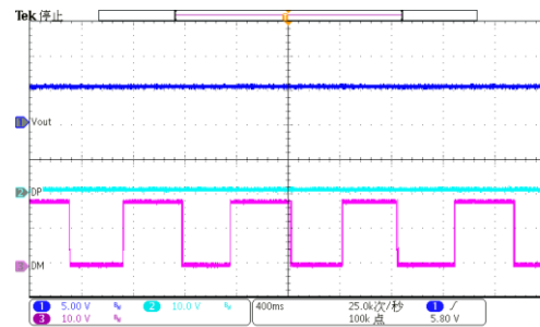
Figure 8-54. DM Short to 18V Battery
