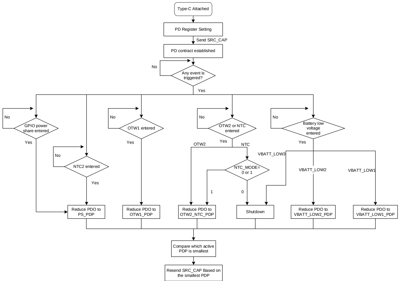
Figure 10-13 PDP State Machine
