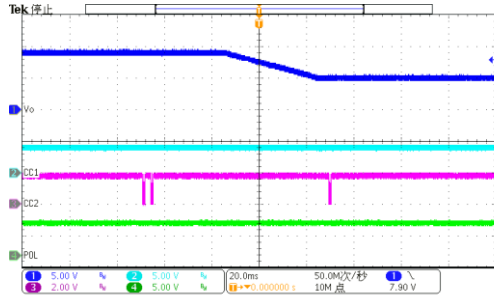
Figure 8-45. PDO Transition 9V-5V
