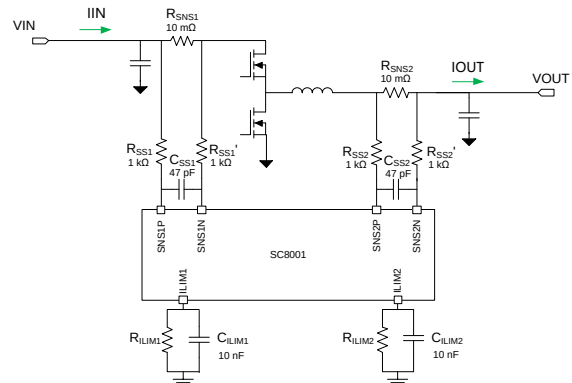
Figure 3 Input/output current monitoring circuit
