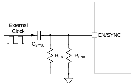
Figure 10-4 EN/SYNC High-pass Filter Demonstration
