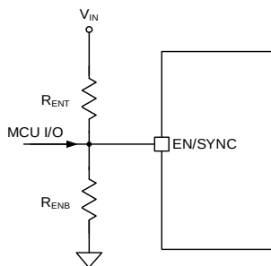
Figure 10-2 EN/SYNC Configuration for Precise Enable
