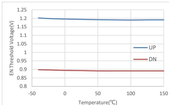
Figure 8-4. Precision Enable Thresholds
