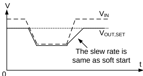
Figure 10-8 Recover from Dropout Operation
