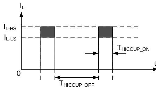
Figure 10-6 Hiccup Mode Operation
