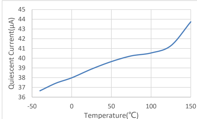
Figure 8-1. Non-Switching Input Supply Current
