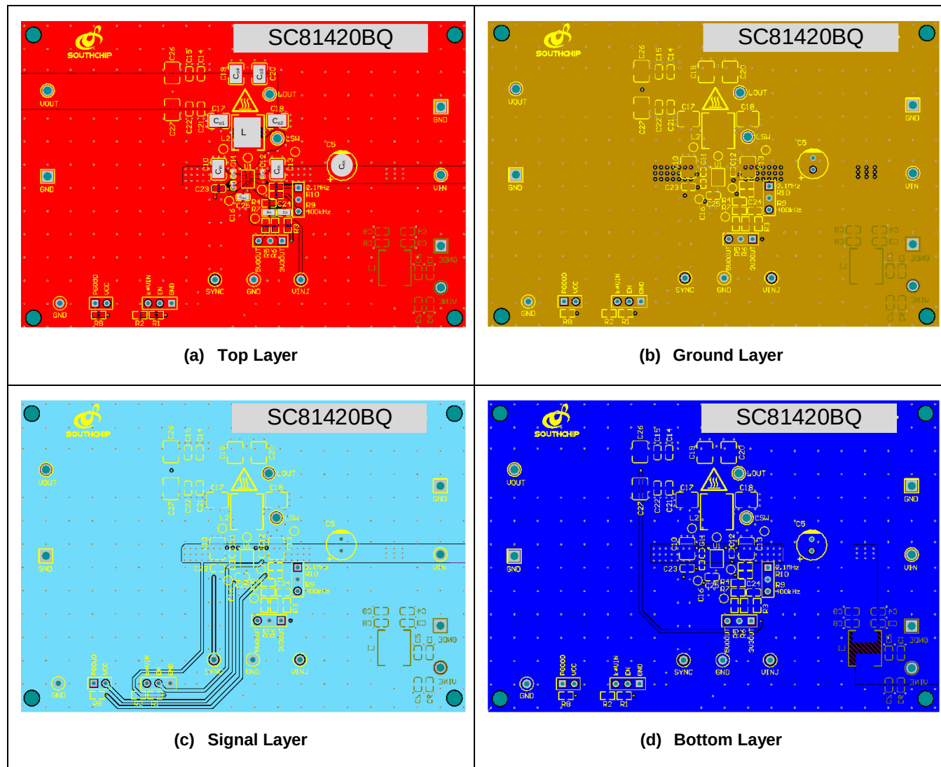
Figure 12-1. Layout Example
