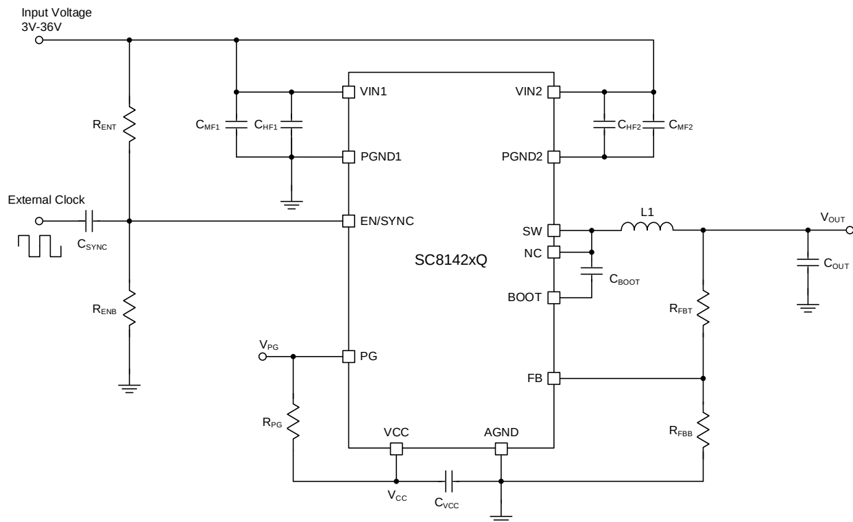
Figure 6-1. Typical Application Circuit of SC81420BQ/SC81420CQ
