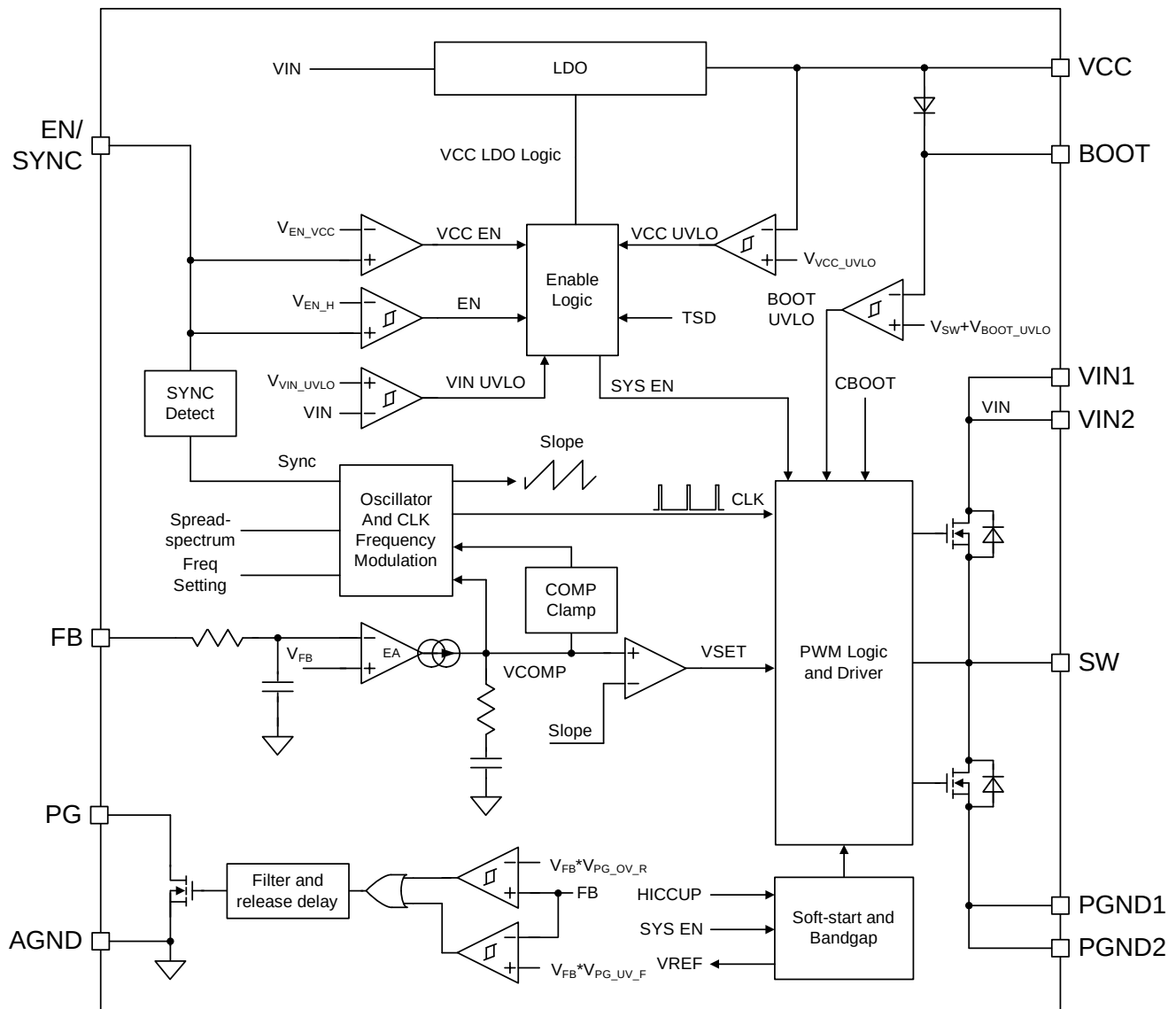
Figure 9-1. SC81420BQ and SC81420CQ Functional Block Diagram
