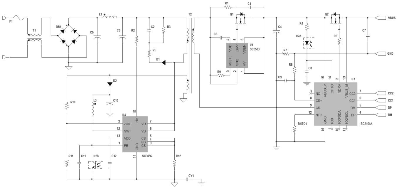
Fig. 1 Typical application circuit
