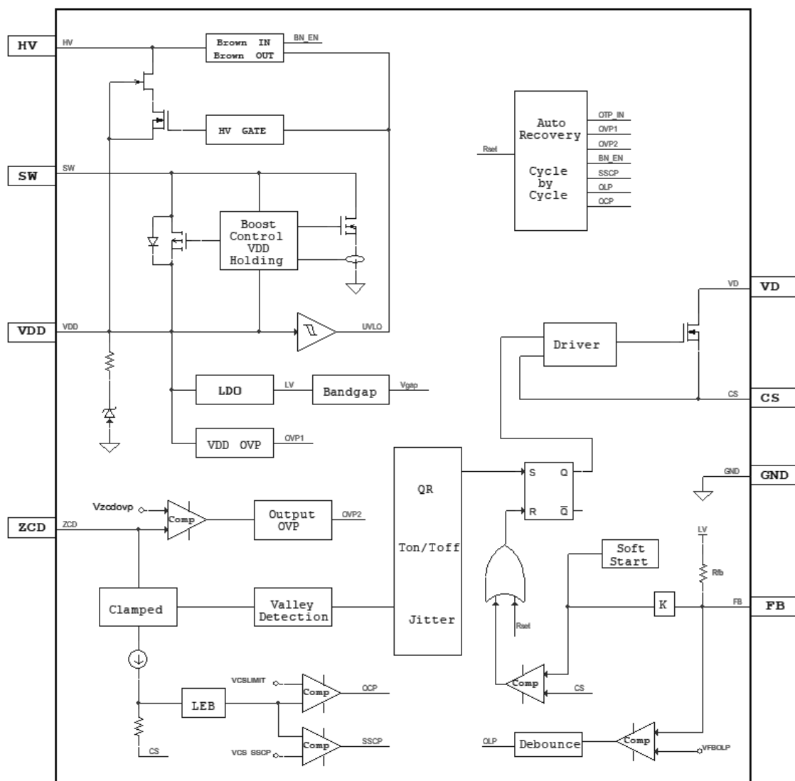
Fig.3 Function Block Diagram
