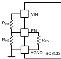
Figure.4 UVLO Threshold Programming
