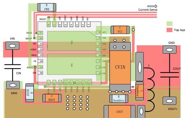
Figure.7 Minimizing the critical path helps mitigate EMI
