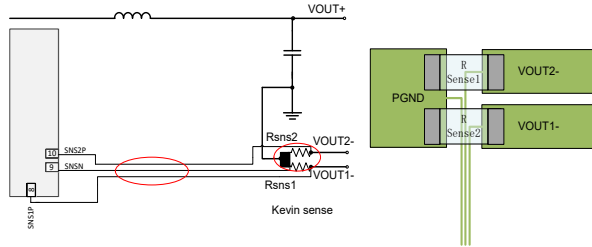
Figure.9 Current sense
