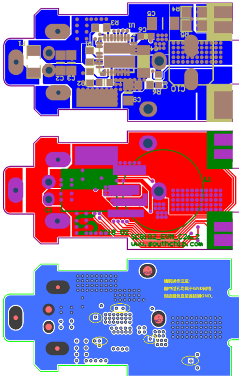
Figure.10 Reference design
