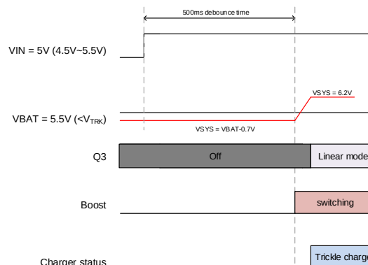
Figure 2 Startup with VBAT < VTRK
