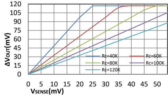
Figure.6 \Delta V_{OUT} vs. V_{SENSE} ( R_{UI}=78\text{ K}\Omega )
