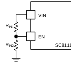
Figure.4 UVLO Threshold Programming
