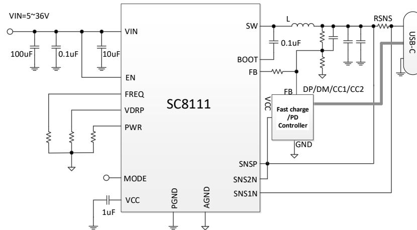
Figure. 2 Typical Application Circuit for Fast charge/PD Application
