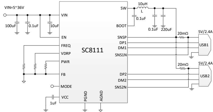
Figure. 1 Typical Application Circuit with 5V4.8A Dual-Outputs
