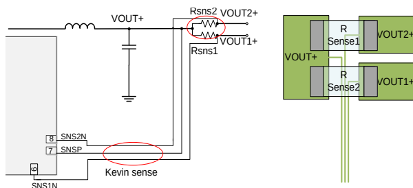
Figure.10 Current sense
