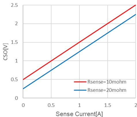
Fig3. CSO Voltage over Sense Current
