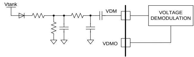
Fig1. Voltage Demodulation
