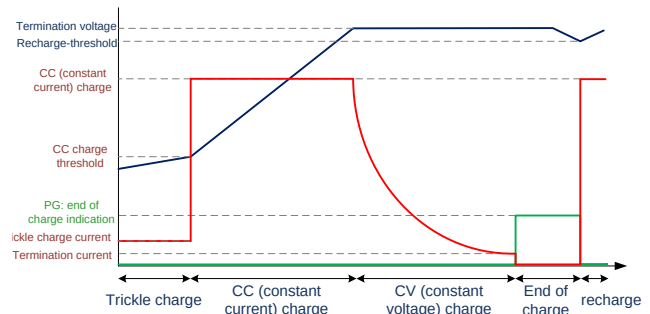
Figure 10. SC8803 Charge curve
