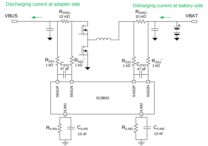
Figure 14 Discharge current monitoring circuit.
