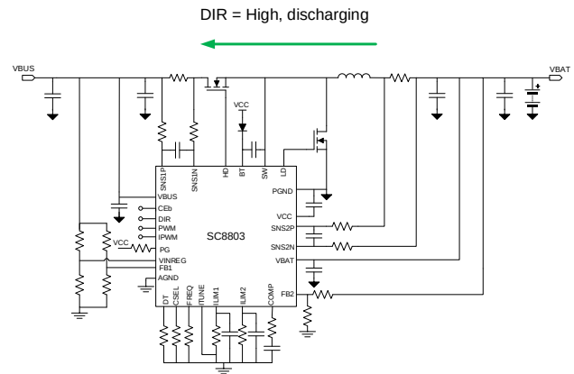
Figure 12 SC8803 Reverse direction discharge mode.
