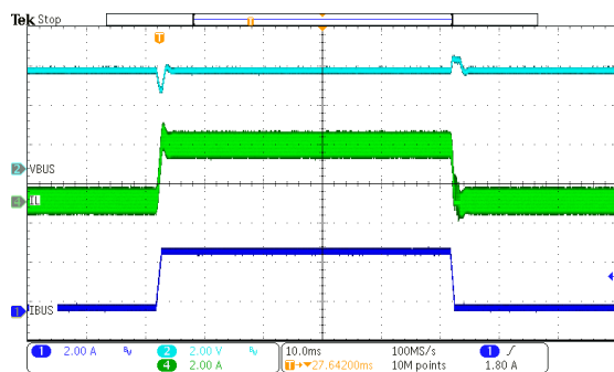
Figure 5. Load trans, VBUS = 5V, 0.5A<—>3A
