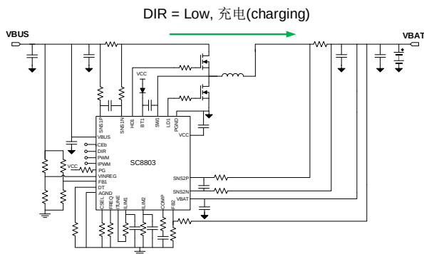
Figure 7. Charging mode when DIR=LOW
