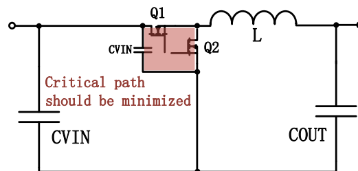
Figure.6 Minimizing the critical path helps mitigate EMI
