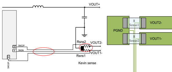
Figure.8 Current sense
