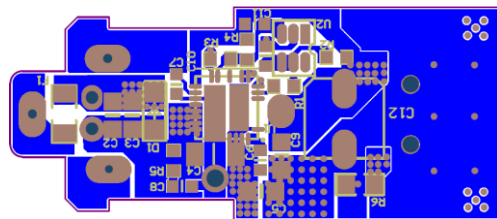
Figure.9 Reference design with internal 5.02V output
