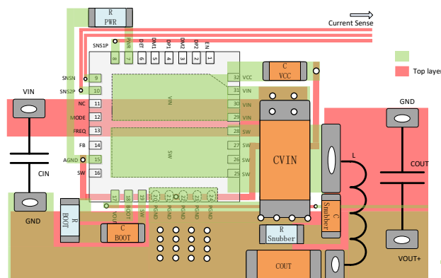
Figure.7 A layout example of SC8103
