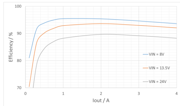
Efficiency Curve
