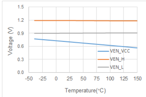
Figure 8-7. Enable Thresholds
