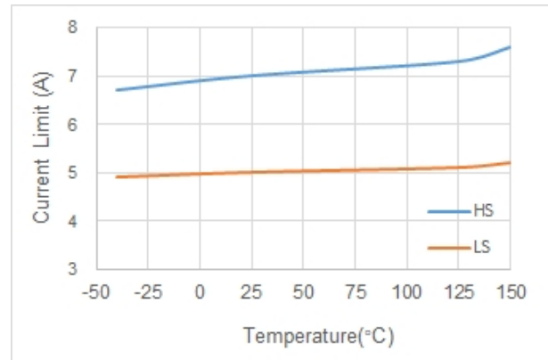
Figure 8-4. High-side and Low-side Current Limits
