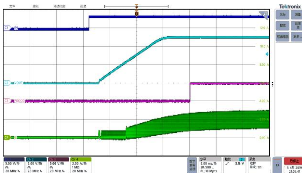
V_{OUT}=5V , F_{SW}=400kHz , MODE=APFM Start-up with 2A Load
