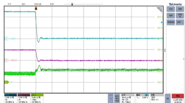
V_{OUT}=5V , F_{SW}=2100kHz , MODE=APFM , I_{OUT}=4A Recovery from Hiccup
