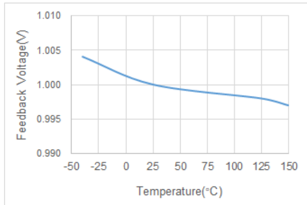
Figure 8-3. Feedback Voltage
