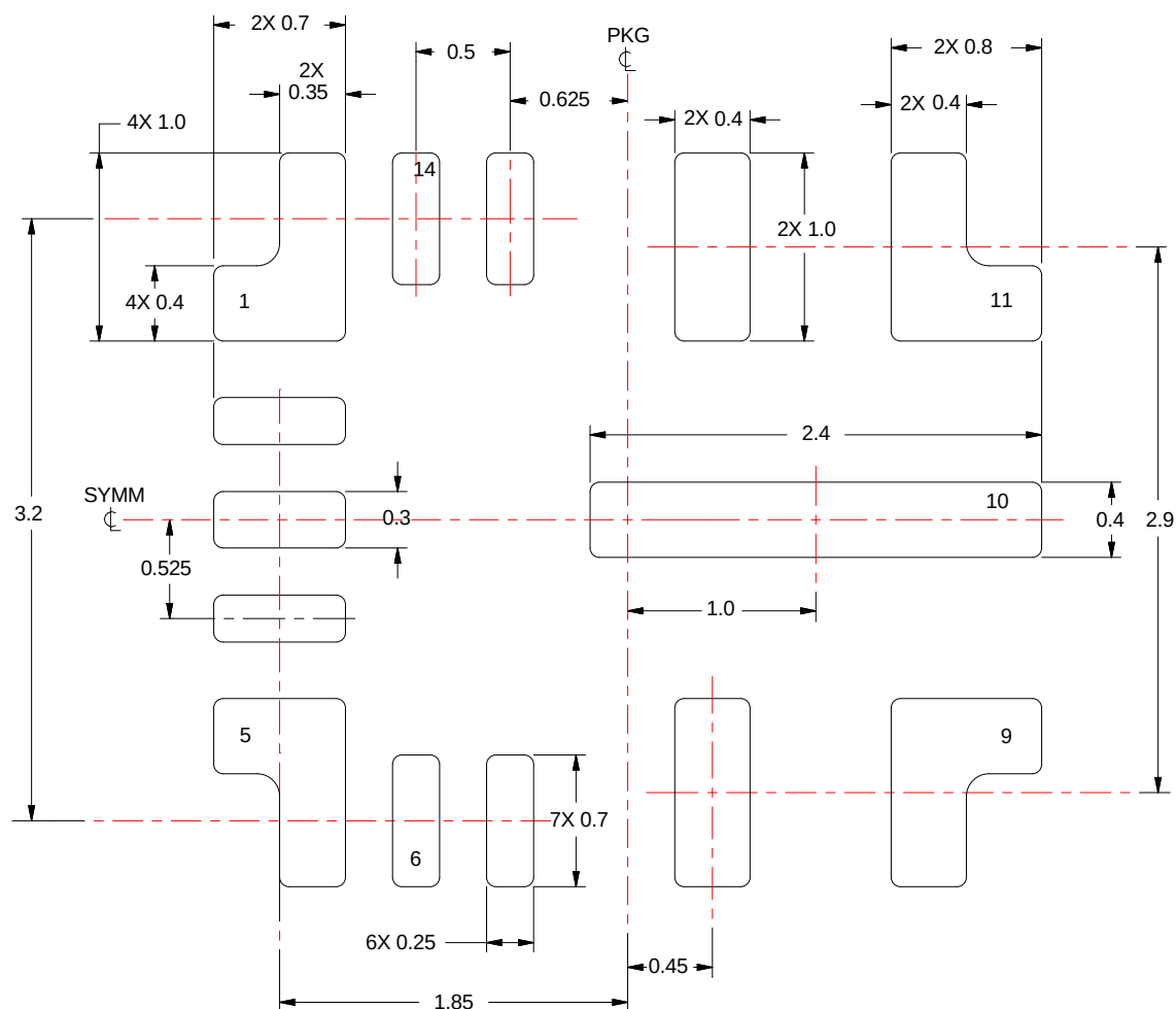
LAND PATTERN
