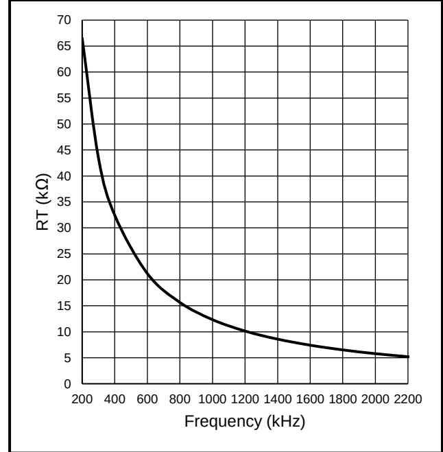
Figure 10-3 RT and Switching Frequency Relationship
