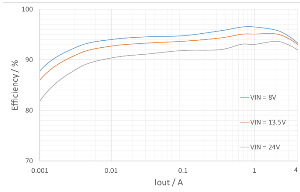
Efficiency Curve
