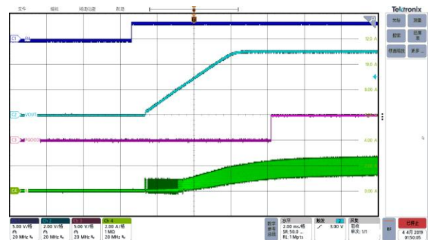
V_{OUT}=5V , F_{SW}=2100kHz , MODE=APFM Start-up with 2A Load
