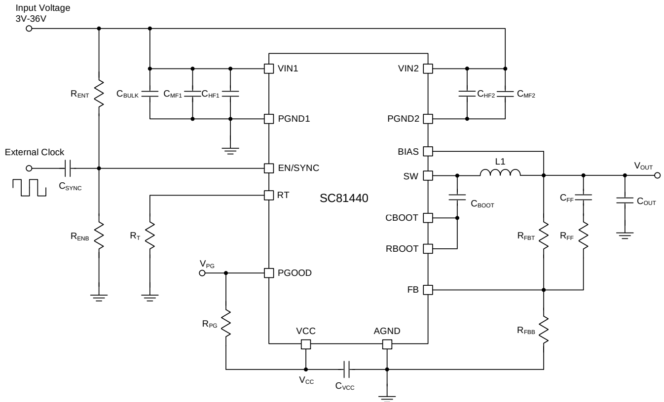
Figure 6-1. Typical Application Circuit
