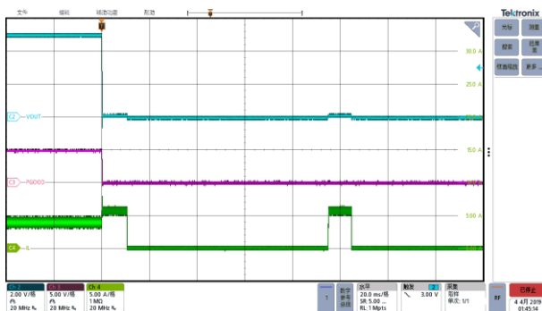
V_{OUT}=5V , F_{SW}=2100kHz , MODE=APFM , I_{OUT}=4A Enter Hiccup
