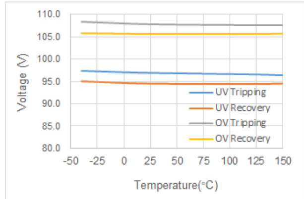
Figure 8-8. PGOOD Thresholds
