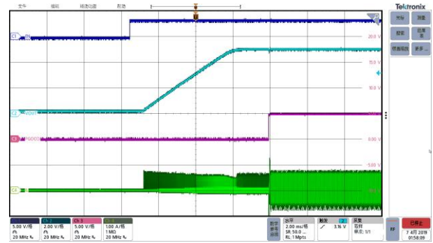
V_{OUT}=5V , F_{SW}=2100kHz , MODE=FPWM Start-up with 50mA Load
