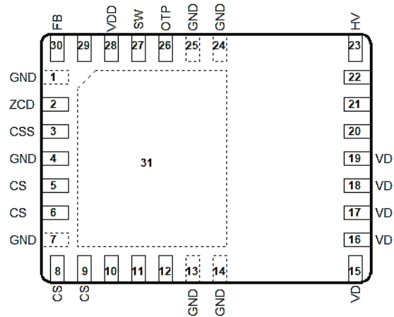
Fig. 2 Top view
